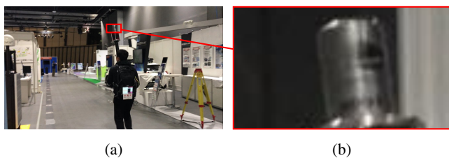
Figure 2: Data collection. (a): the scene of data collection. (b): the working Velodyne HDL-32E sensor
